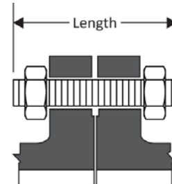
Stud Bolt with Nuts
